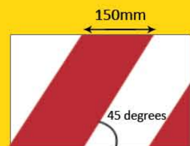
Examples of fluorescent retroreflective sheeting strips on skip
