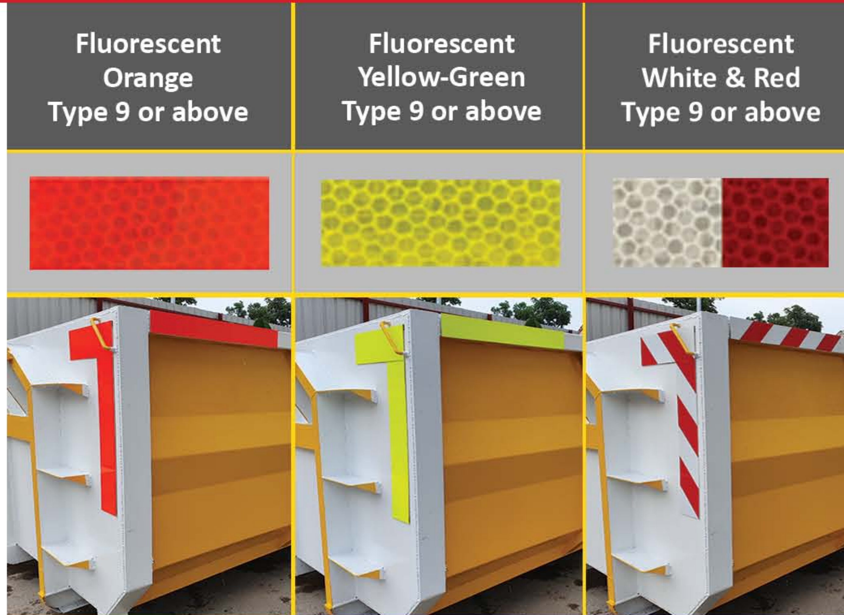
Examples of fluorescent retroreflective sheeting strips on skip
