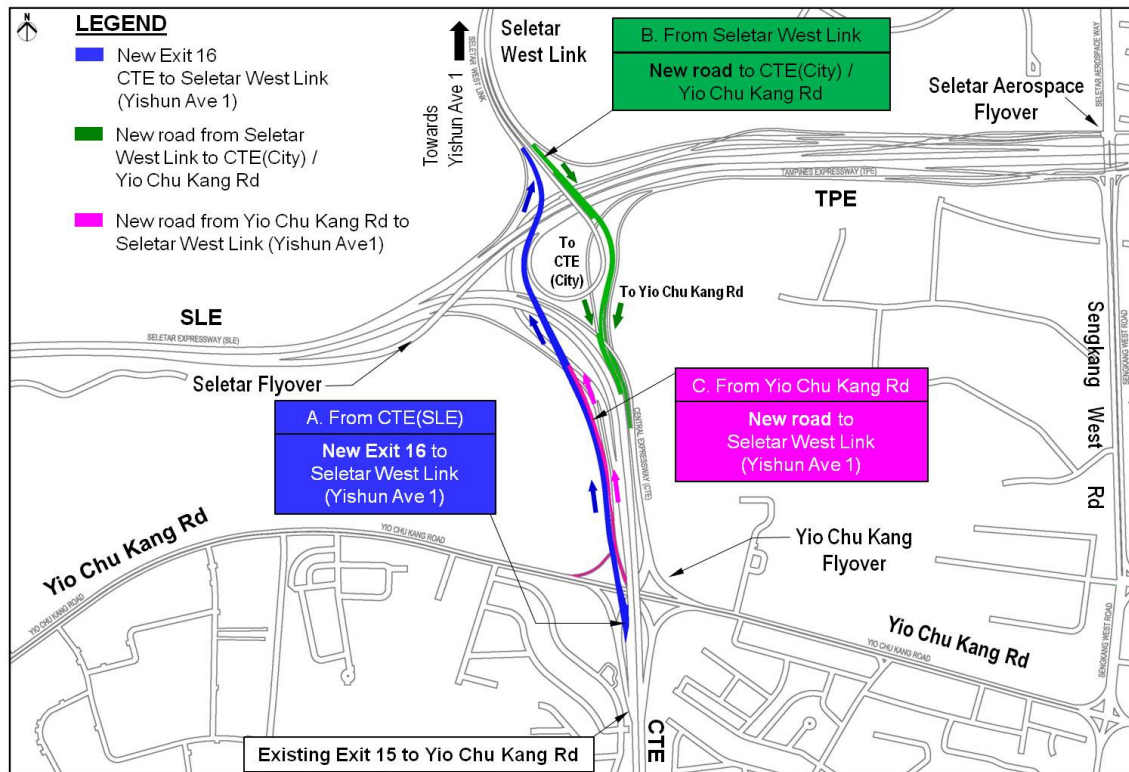
ER391 – EXPANSION OF CTE/TPE/SLE INTERCHANGE LOCATION PLAN FOR NEW FLYOVER FROM CTE TO SELETAR WEST LINK(YISHUN AVE 1), NEW SLIP ROAD FROM YIO CHU KANG ROAD TO SELETAR WEST LINK(YISHUN AVE 1) & SELETAR WEST LINK TO CTE(CITY) & YIO CHU KANG ROAD
