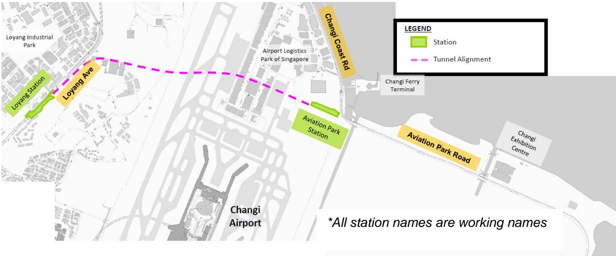
Location map of tunnel between Aviation Park Station and Loyang Station
