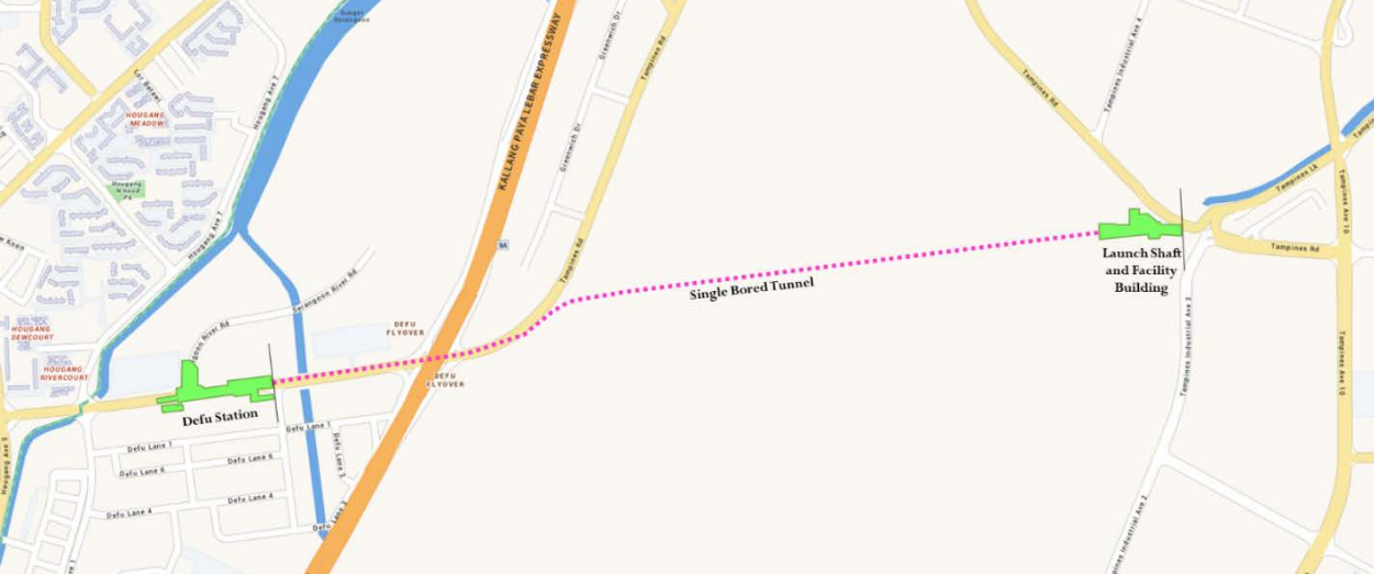
Location map of tunnel between Tampines North and Defu stations
