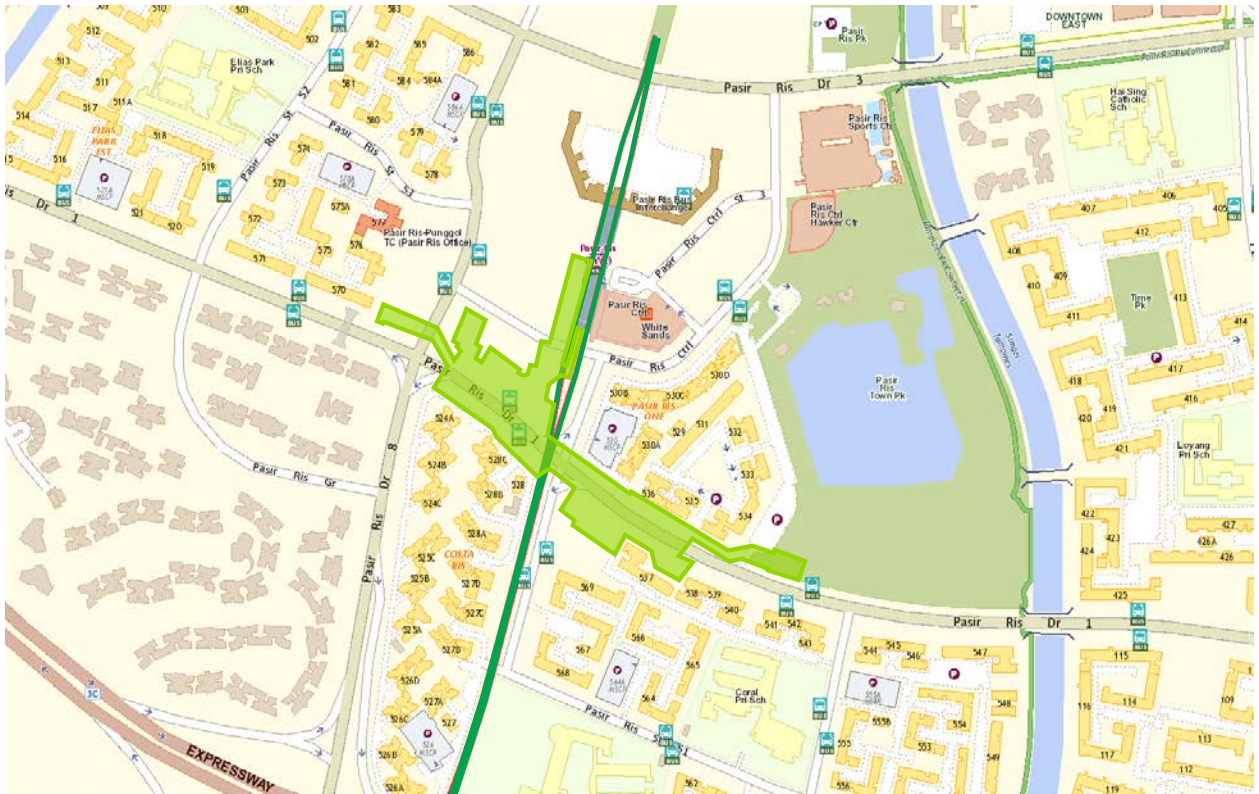
Location of CRL Pasir Ris Station
