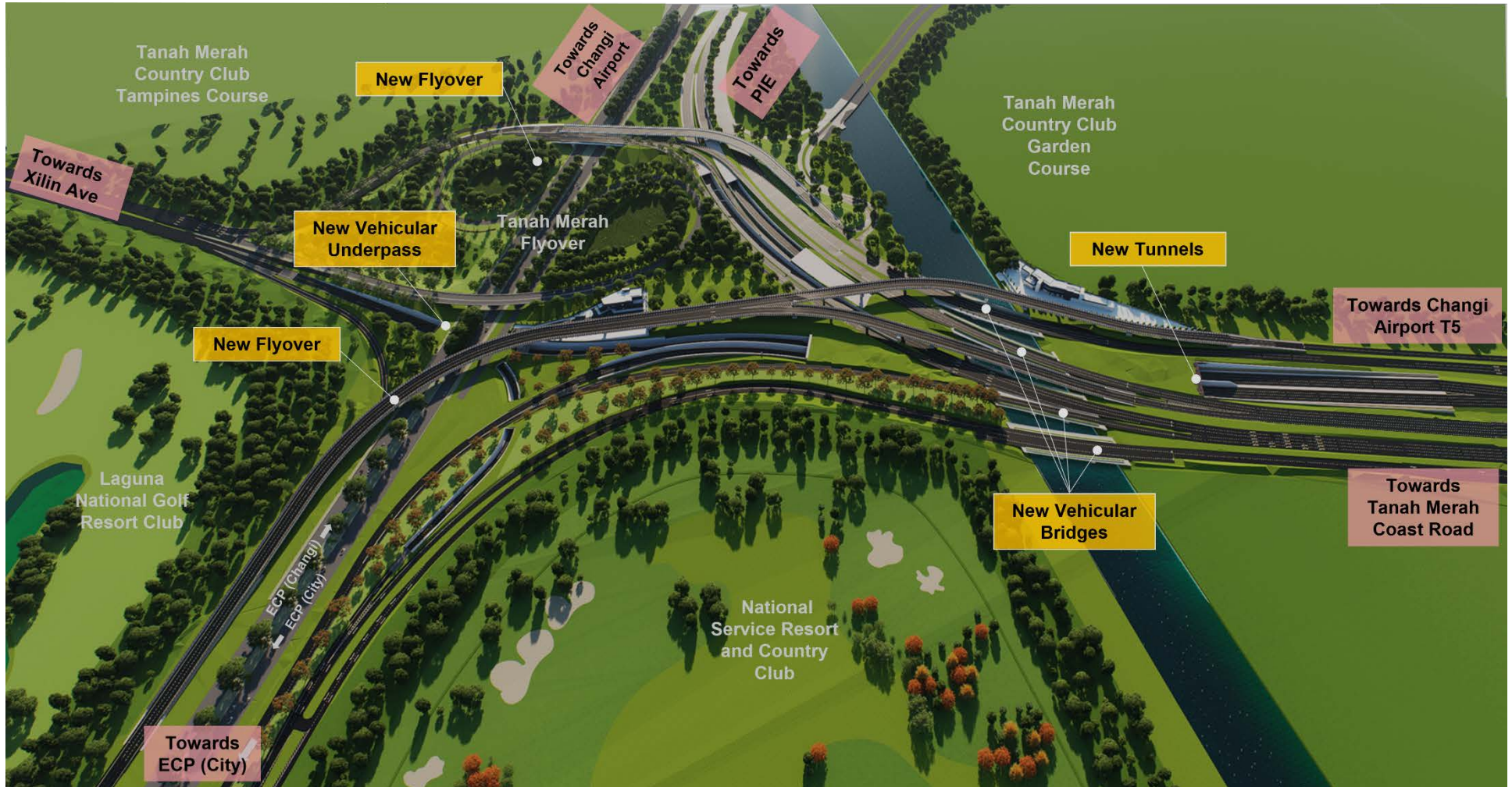
Artists' Impression of Enhancement of Xilin Ave/ECP/Tanah Merah Flyover Interchange/Tanah Merah Coast Road
