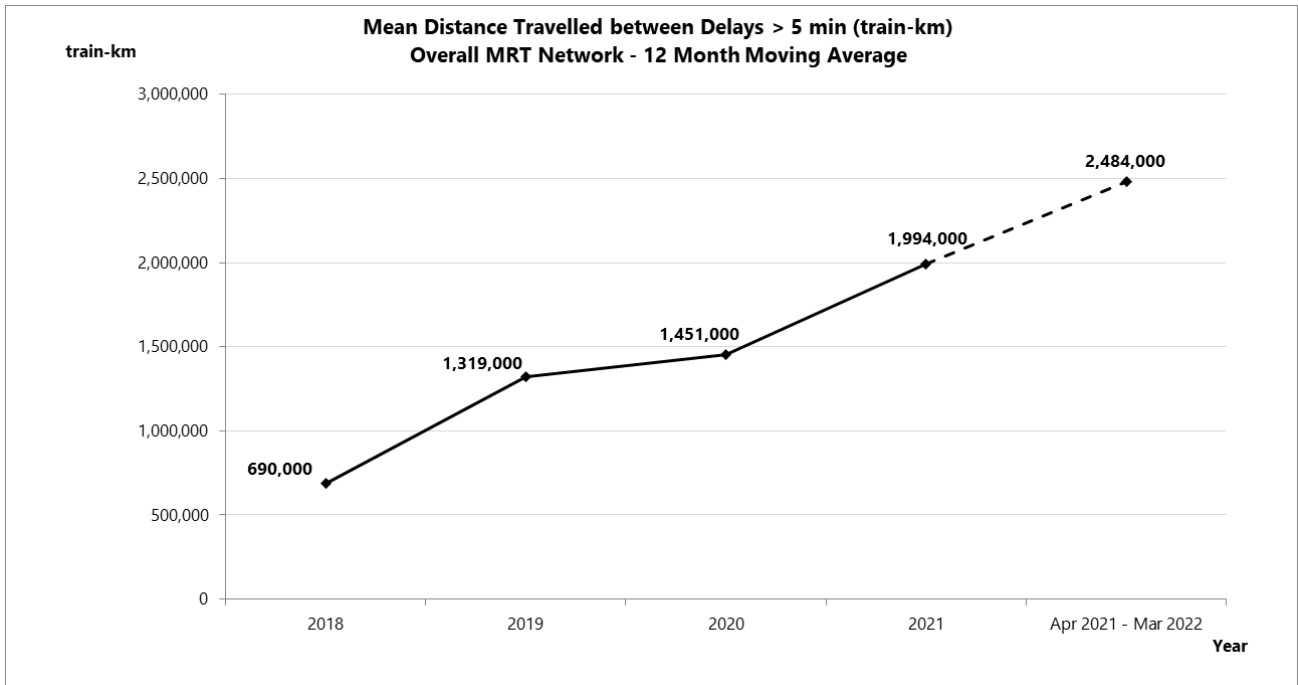
Figure 1: Mean Distance Travelled between Delays > 5 min (train-km) for Overall MRT Network – 12 Month Moving Average
