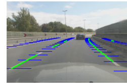
Lane Detection
